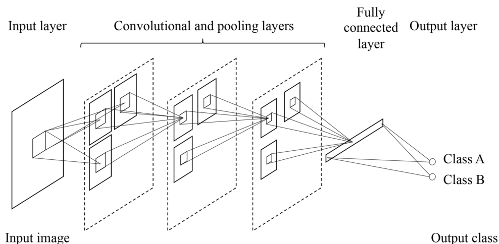
Fig. 5 Architecture of a CNN. The layers in the CNN are connected with local shift-invariant inter-connections (or convolution with a local kernel). The input and output of the CNN are images and class labels (e.g., Class A and Class B), respectively
